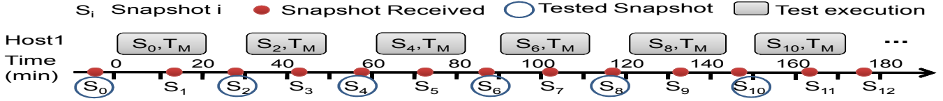
Figure 2: Actual execution timeline, in minutes, of a testing plan in Amulet for Example 1 from Table 1. Each box denotes a run of the mysamchk ( T_M ) test on the respective snapshot S_i . The horizontal width of each box corresponds to the test execution time.
