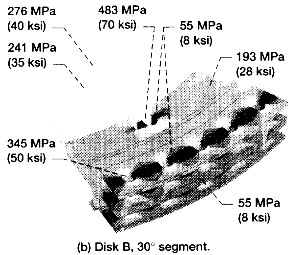
Figure 5.—Maximum shear stress profiles for rim-loaded compressor disks based on finite-element analysis. Speed, 11 200 rpm.
