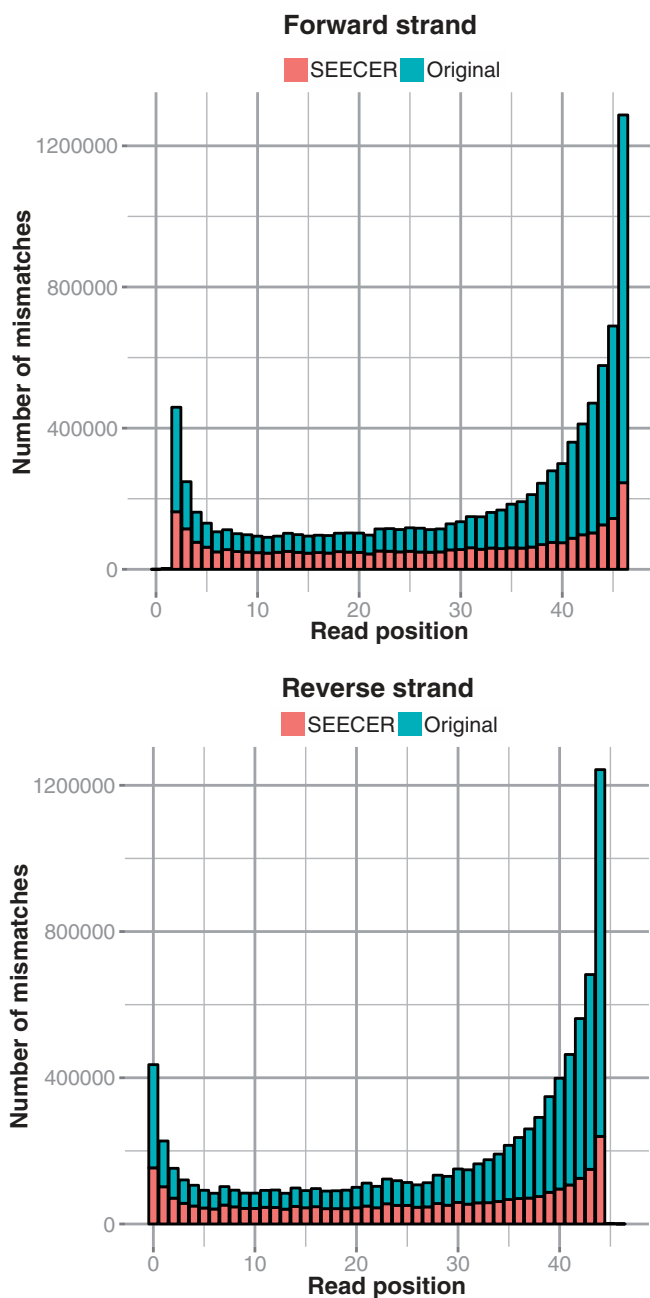
Figure 2. The distribution of mismatches to the reference of pair-mapped reads (using TopHat alignment) of the 55M paired-end 45bp reads of human T cells dataset: only reads that are aligned both before and after error correction are shown.
