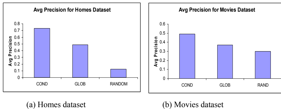
Figure 5: Average Precision
