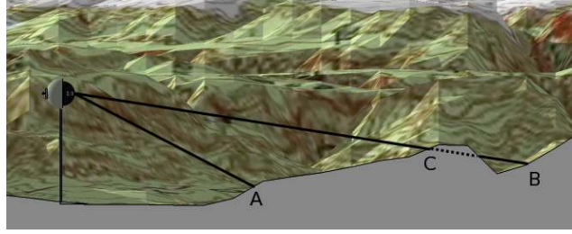
Figure 2: The effect of visibility function. Here sensor and point A are inter-visible, therefore v(s_i, \mathbf{A}) = 1 , but it is not the case for s_i and B , because the line-of-sight is obscured at point C .
