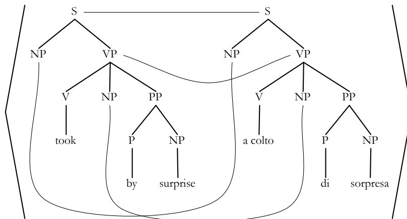
Figure 1: A synchronous tree pair.
