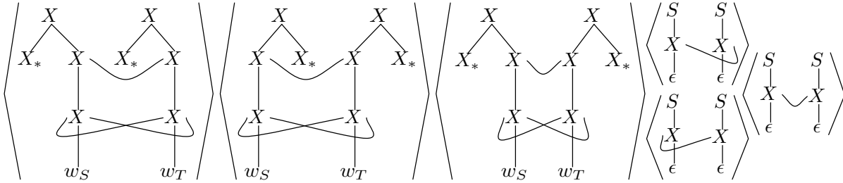
Figure 2: A normal form for synchronous tree-insertion grammar. (Reproduced from Nesson et al. (2006).)
