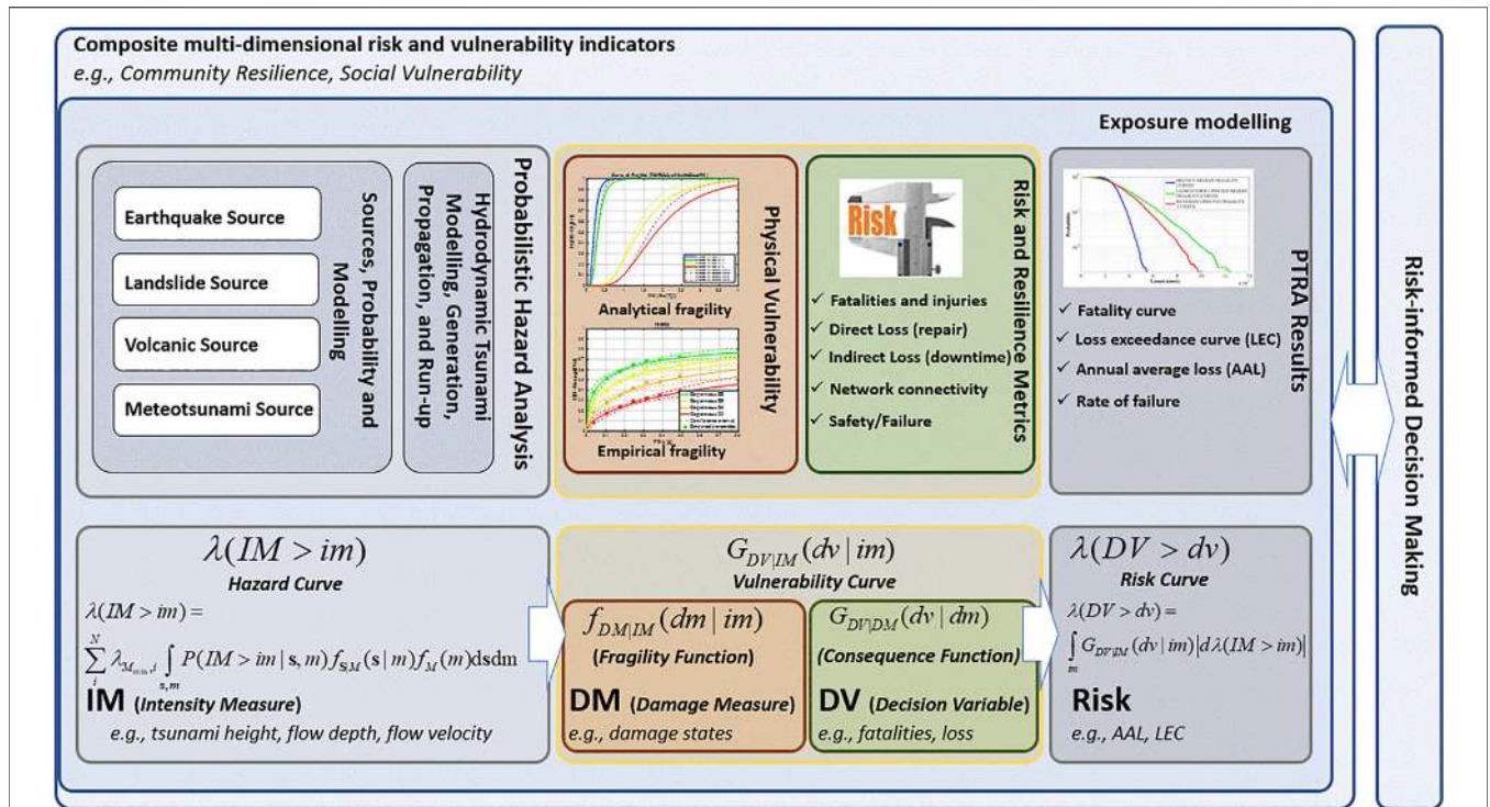
FIGURE 1 | Roadmap of PTHA and PTRAs frameworks: The entire process of risk evaluation needs to interact with the (risk-informed) decision-making process. Composite multi-dimensional risk and vulnerability indicators (“Probabilistic Tsunami Hazard Analysis” section) are shown as defining the context for the complex tsunami risk evaluation. The exposure modeling (“Probabilistic Tsunami Risk Assessment” section) defines groups of individuals and assets at risk. The horizontal flowchart at the bottom of the figure shows the PEER-like workflow for risk assessment. Probabilistic hazard analysis (“Probabilistic Tsunami Hazard Analysis” section) discusses estimation of the mean annual frequency (rate) of exceedance of a given value ( im ) of an intensity measure ( IM , Eq. 1) commonly visualized as a hazard curve. The IM can be a vector or a scalar that describes the intensity of a tsunami. Examples of IM ’s are flow depth, maximum tsunami inundation height, etc. M refers in a generic manner to the size of various tsunami sources (e.g., earthquake magnitude, landslide volume). The tsunami sources, probability and modeling (earthquake, landslide, volcanic and meteotsunami) are discussed in “Probabilistic Tsunami Hazard Analysis” section. s denotes the vector of source parameters. N denotes the number of tsunamigenic sources. \lambda_{M_{min,i}} denotes the mean annual frequency of tsunamigenic events exceeding M_{min} from source i . “Gaps in Hydrodynamic Tsunami Modeling, Generation, Propagation, and Run-up” section discusses hydrodynamic tsunami modeling, generation, propagation and run-up. The physical vulnerability (“Gaps in Physical Vulnerability” section) discusses the estimation of the probability distribution for a damage measure ( DM , specific value dm ) given IM (specific value im ), known as the fragility function. The most common example of a DM is the physical damage state. The risk and resilience metrics section (“Gaps in Risk and Resilience Metrics” section) discusses the estimation of various decision variables (e.g., fatalities, repair costs, downtime) denoted as DV (specific value dv ). More specifically, it discusses the probability distribution for DV given DM also known as the consequence function. The vulnerability function (Eq. 3) describes the (mean and standard deviation) of the probability distribution for DV given IM and is obtained by integrating over the entire domain of DM . One way to show the PTRAs results is through visualizing the mean annual frequency of exceeding a specific value dv of DV (e.g., the loss exceedance curve (LEC) or the annual average loss (AAC)) shown in Eq. 2, referred to generically as the risk curve.
