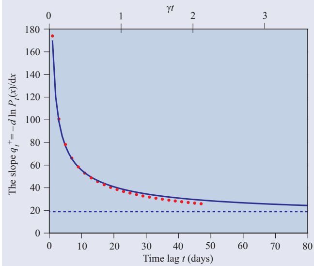
Figure 6. Solid curve: the slope q_t^\pm = -d \ln P/dx of the exponential tail for x > 0 as a function of time. Points: the asymptotic approximation (46) for the slope in the limit \gamma t \ll 2 . Dashed line: the saturation value q_*^\pm of q_t^\pm for \gamma t \gg 2 , equation (45).
