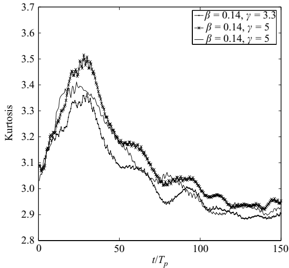
FIGURE 14. The kurtosis for the cases in figures 11–13.
