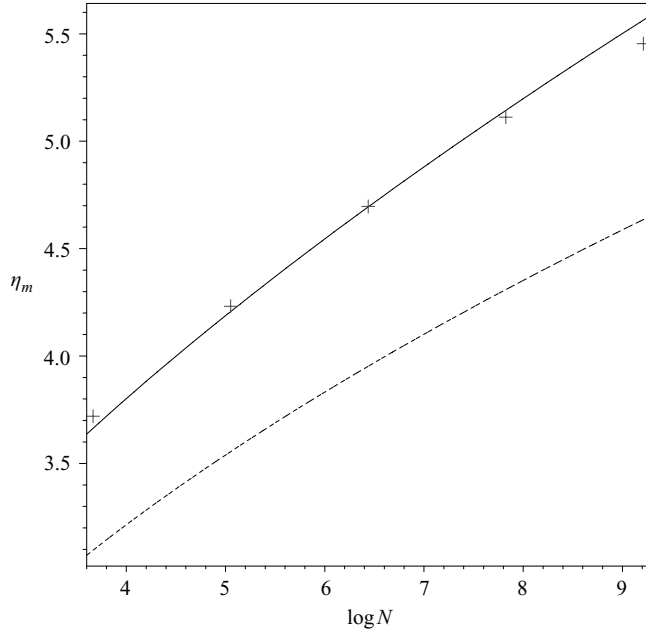
FIGURE 10. The average largest surface elevation of scenes containing N waves. Simulations, case A, (crosses) are compared with the expected value given by equation (19) for \sigma = 0.071 used in the simulations (solid), and \sigma = 0 corresponding to the Gaussian case (dashed).
