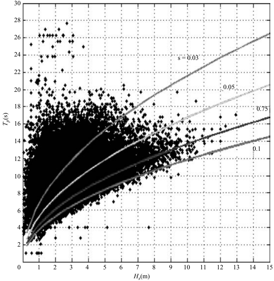
FIGURE 2. Scatter diagram for H_s and T_p from the northern North Sea. Pooled data 1973–2001, from the platforms Brent, Statfjord, Gullfax and Troll. Curves of constant steepness s are also shown. The figure was prepared by K. Johannessen Statoil.
