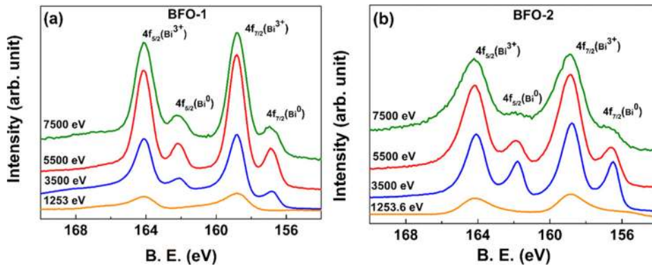
FIG. 3. Bi 4f spectra of BFO-1 (a) and BFO-2 (b) obtained using the Mg K\alpha (1253.6 eV) source along with HXPES.
