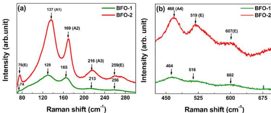
FIG. 2. Raman spectra of BFO-1 and BFO-2 showing shifting of modes due to increment in particle size in region 70–300 cm -1 (a) and 425–700 cm -1 (b).
