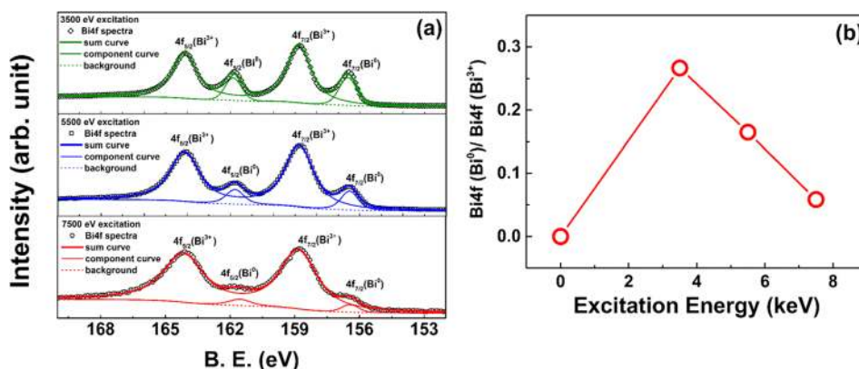
FIG. 4. Peak fitting analysis of HXPES spectra for Bi 4f region (a) and ratio of Bi 4f(\text{Bi}^0) and Bi 4f(\text{Bi}^{3+}) as a function of excitation energy (b) for sample BFO-2.
