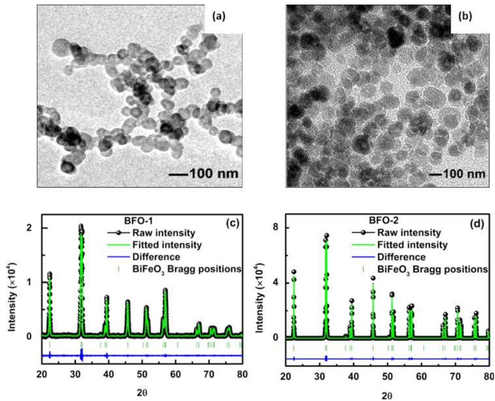
FIG. 1. TEM of BFO-1 and BFO-2 ((a) and (b)) and Rietveld refined XRD pattern of BFO-1 and BFO-2 ((c) and (d)).
