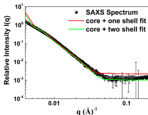
FIG. 5. Circle ( \circ ) shows the SAXS spectrum of BFO-2 NPs, having \sim 155 nm diameter, with 25% polydispersity. Red line shows a model fitting with one core and one shell. Green line shows a model fitting with one core and two outer shells. The fitting has been carried out using nonlinear least-squares fit under the IGOR platform. Here, the scattering wavevector q = 4\pi\lambda^{-1}\sin\theta is defined by X-ray wavelength \lambda and scattering angle 2\theta .
