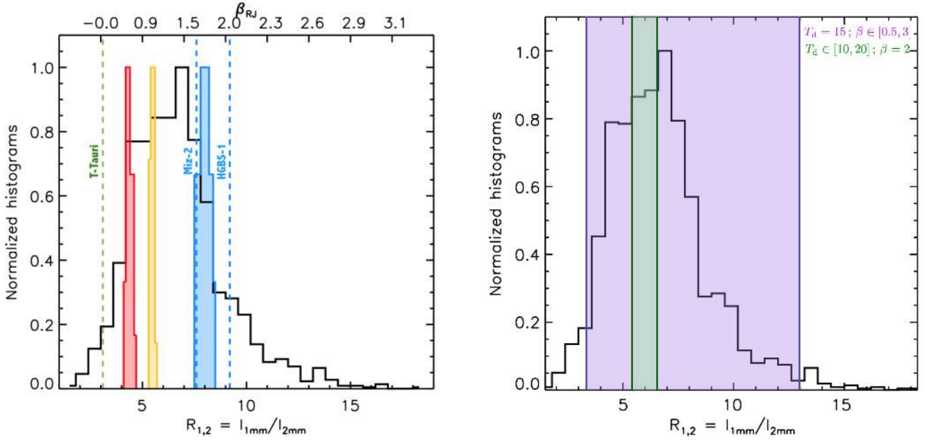
Fig. 4. Left: normalized histogram of R_{1,2} in black for all the unmasked pixels in the maps. The colored normalized histograms represent the R_{1,2} distributions within one-beam area ( 24'' ) around the central coordinates (see Table 1) of K04166 (red), K04169 (yellow), and Miz-8b (blue). The vertical dashed lines refer to the value of the ratio at the peak-intensity position of T Tauri (green), Miz-2, and HGBS-1 (blue). The upper x -axis shows the corresponding \beta values in the Rayleigh-Jeans limit (see Sect. 5.1). Right: same as in the left panel with shades that now represent ranges of R_{1,2} corresponding to graybodies with 1) a constant temperature T_d of 15 K but a varying \beta between 0.5 and 3 in purple; 2) a constant \beta of 2, but varying T_d between 10 K and 20 K in green.
