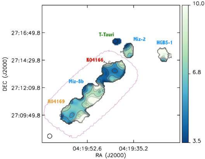
Fig. 3. Ratio map between the two NIKA bands, R_{1,2} = \frac{I_{1 \text{ mm}}}{I_{2 \text{ mm}}} . The unmasked region corresponds to a signal-to-noise ratio on the fluxes above 10 at both wavelengths. Black contours represent R_{1,2} equal to 3, 4.5, 5.6, 7, 8, and 9. The purple contour corresponds to the part of the field with homogeneous observing time >240 s per pixel (see Fig. A.1). The open circle in the bottom left corner represents the beam size ( 24'' ).
