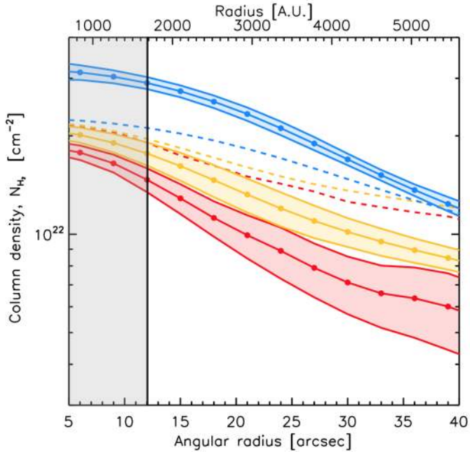
Fig. 6. Radial N_{\text{H}_2} column density profiles for K04166 (red), K04169 (yellow), and Miz-8b (blue), as derived from Herschel Gould Belt survey data. The color-code is the same as in Fig. 5, as is the gray-shaded area.
