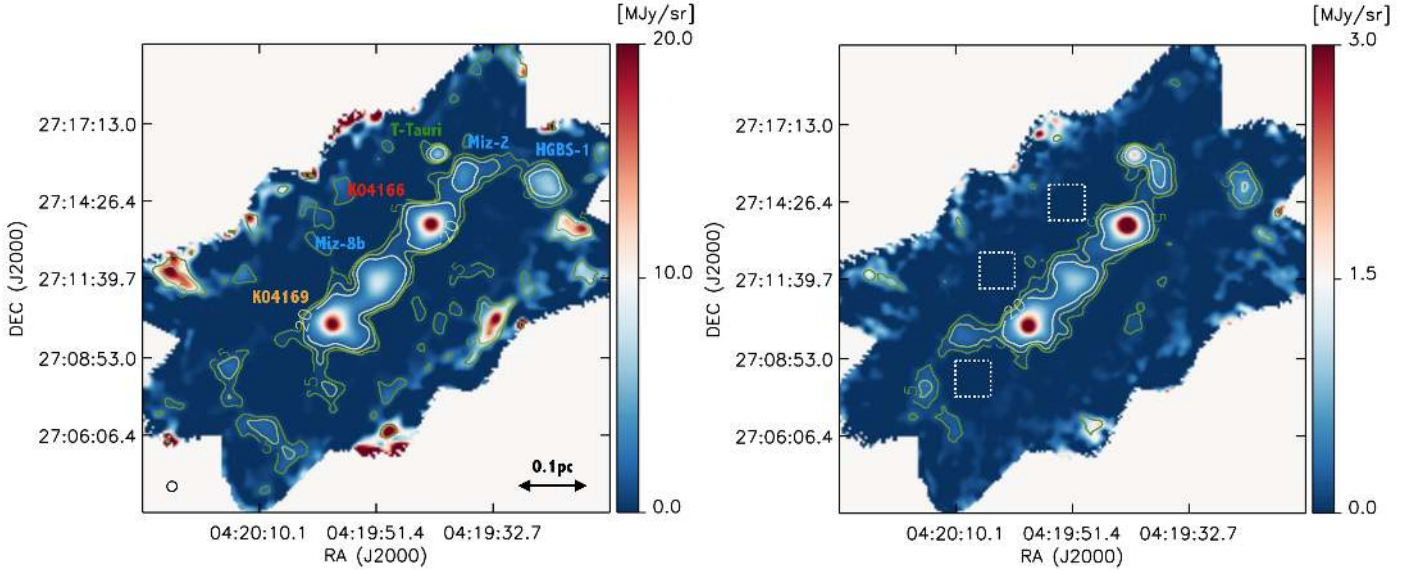
Fig. 1. Dust continuum maps of a portion of the B213 filament obtained with the NIKA camera on the IRAM 30 m telescope at 1.15 mm ( left panel ) and 2 mm ( right panel ). The two maps are shown after smoothing to a common resolution of 24'' (see the circle in the bottom-left corner of the left panel). The green contours represent the signal-to-noise ratio levels (5, 10, 20) at each wavelength. The labels in the left panel correspond to the sources analyzed in this work, which are listed in Table 1. The three squares on the right delimit the regions where we estimate the rms intensity of the two maps at 24'', which corresponds to 0.75 MJy/sr and 0.09 MJy/sr at 1.15 mm and 2 mm respectively.
