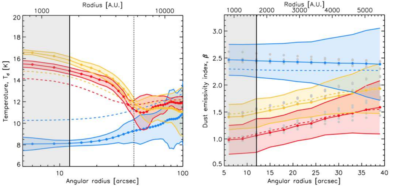
Fig. 5. Left: dust temperature radial profiles of K04166 (red), K04169 (yellow), and Miz-8b (blue). The dust temperatures were derived from Herschel Gould Belt survey data 1 . The dashed colored lines correspond to line-of-sight averaged temperatures obtained from direct SED fitting, while dots and solid lines correspond to Abel-reconstructed dust temperatures. The colored shades represent the 1\sigma errors of the Abel-reconstructed temperatures. Right: radial profiles of \beta using the Abel-reconstructed temperatures. The color-code is the same as in the left panel. The gray dots show the \beta profiles corresponding to four different versions of the maps used to quantify systematic effects due to spatial filtering in the data. The gray-shaded area in both panels indicates radial distances below the half-beam width of 12'' . The Abel transform is only performed for radial distances smaller than the dotted black vertical line in the left panel. On the upper x-axis the radial distance is in astronomical units assuming a distance of 140pc for the Taurus molecular cloud.
