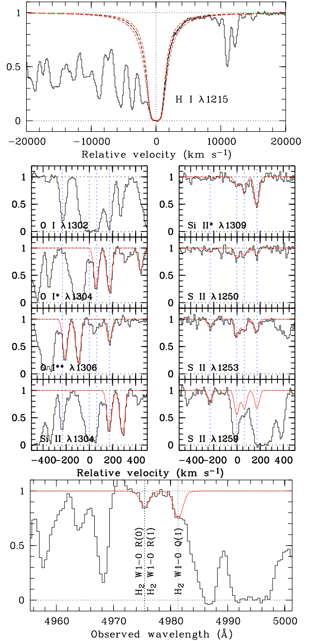
Fig. 1. Upper panel: section of the LR afterglow spectrum showing the DLA line at the GRB redshift, z_{\text{abs}} = 4.048 . Overlaid is the best fitting DLA profile, corresponding to \log N(\text{H I}) = 20.85 \pm 0.10 . Middle panel: fits to the O I, O I*, O I**, Si II, Si II*, and S II lines in the MR spectrum. The zero-point for the velocity scale is z_{\text{abs}} = 4.048 . Lower panel: the likely H _2 lines at the GRB redshift in the MR spectrum.
