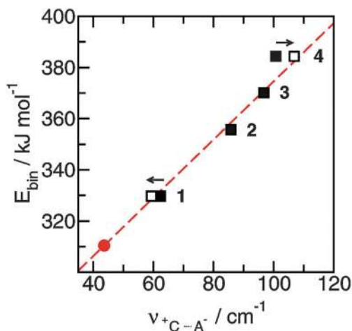
Fig. 7 Average binding energies E_{\text{bin}} per ion pair in tetramers of the ionic liquids 1–4 plotted versus the measured H-bond frequencies \nu_{\text{C-A}} . Using the obtained linear relationship we can predict the H-bond frequency for ionic liquid ([1,2,3,4,5-pentamethyl-im][NTf 2 ]) (filled circle). The filled symbols represent the measured frequencies and the open symbols give the frequencies corrected for the reduced masses. Reprinted from ref. 52 with permission. Copyright 2010 Wiley VCH.
