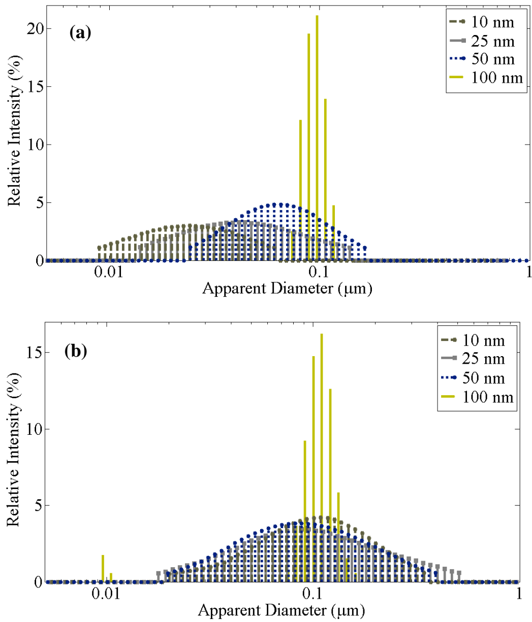
Fig. 2. Differential scattered light intensities from gold nanoparticles of 5 μg/ml concentration suspended in DI water (a), DMEM (b). Measurements were conducted at 37°C
