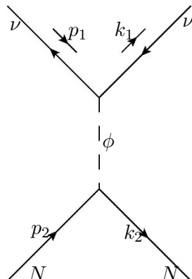
Figure 7. The Feynman diagram of coherent \bar{\nu}N scattering mediated by the new light scalar boson.
