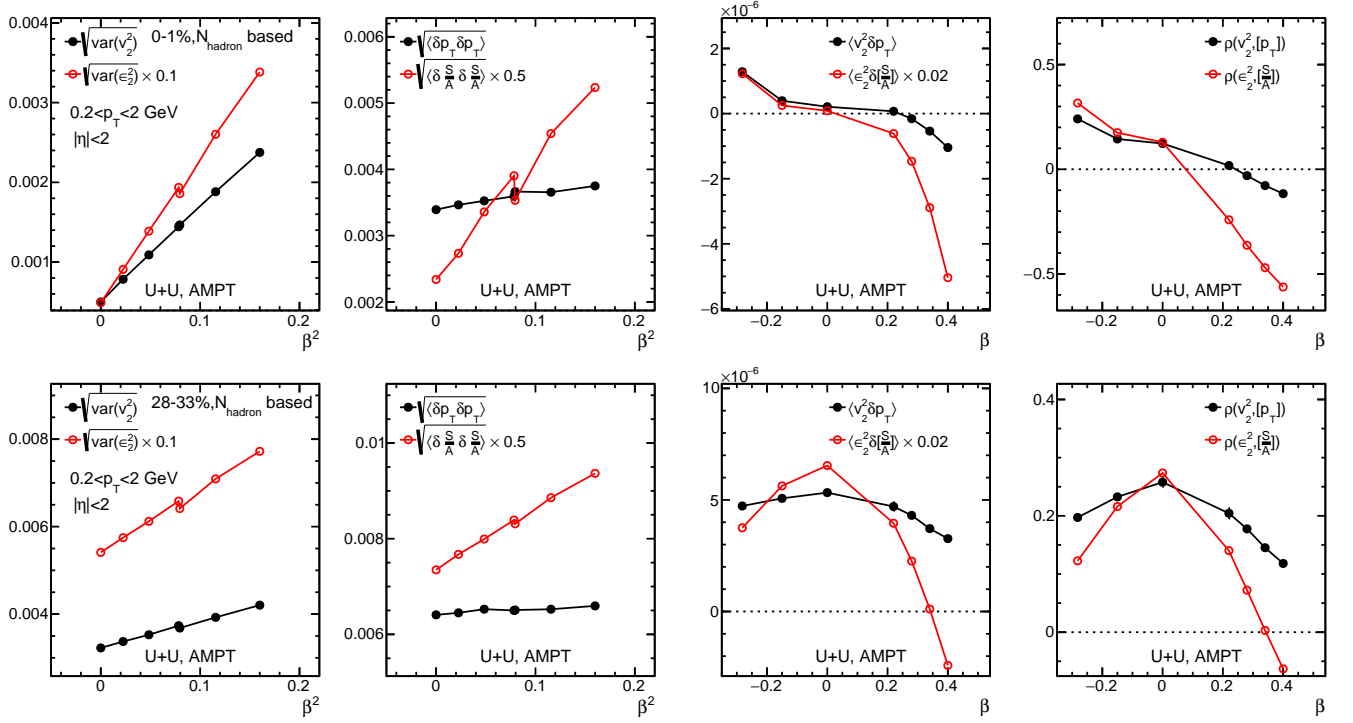
FIG. 9: The \beta^2 dependence of various quantities for the v_2 - [p_T] correlation (solid circles) and the \varepsilon_2 - S/A correlation (open circles) in the top 0–1% centrality (top row) and 28–33% centrality (bottom row) based on the N_{\text{hadron}}(|\eta| < 1) event classes. The data points for \beta = -0.28 are shifted slightly to the right of the data points for \beta = 0.28 .
