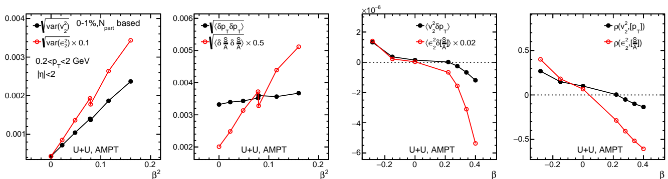
FIG. 3: The \beta^2 dependence of various quantities involved in v_2 - [p_T] correlation (solid circles) and \varepsilon_2 - S/A correlation (open circles) in top 0–1% centrality based on the N_{\text{part}} event class. The data points for \beta = -0.28 are shifted slightly to the right of the data points for \beta = 0.28 .
