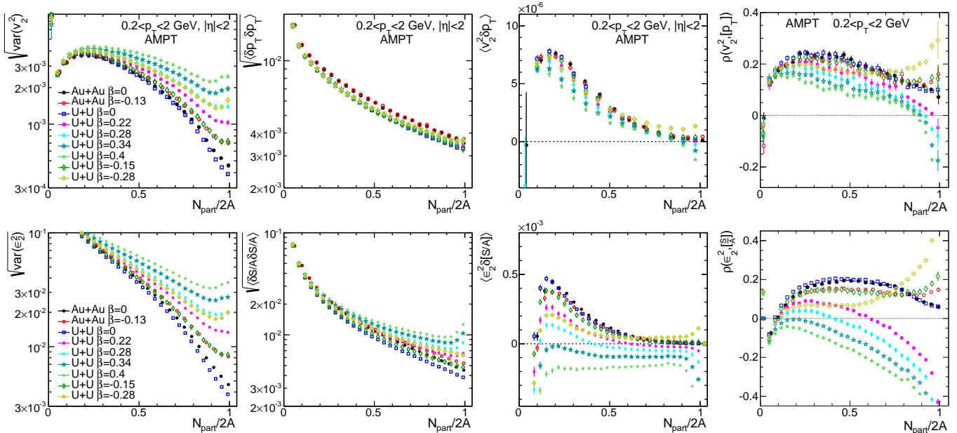
FIG. 2: The N_{\text{part}} dependence of v_2^2 variance (top-left), [p_T] variance (2nd from top-left), flow- [p_T] covariance \langle v_2^2 \delta p_T \rangle (3rd from top-left) and Pearson coefficients \rho(v_2^2, [p_T]) (top-right) in Au+Au and U+U collisions with different deformation parameter \beta . The bottom panels show the corresponding initial-state estimators in the Glauber model. The event class used for averaging is based on N_{\text{part}} .
