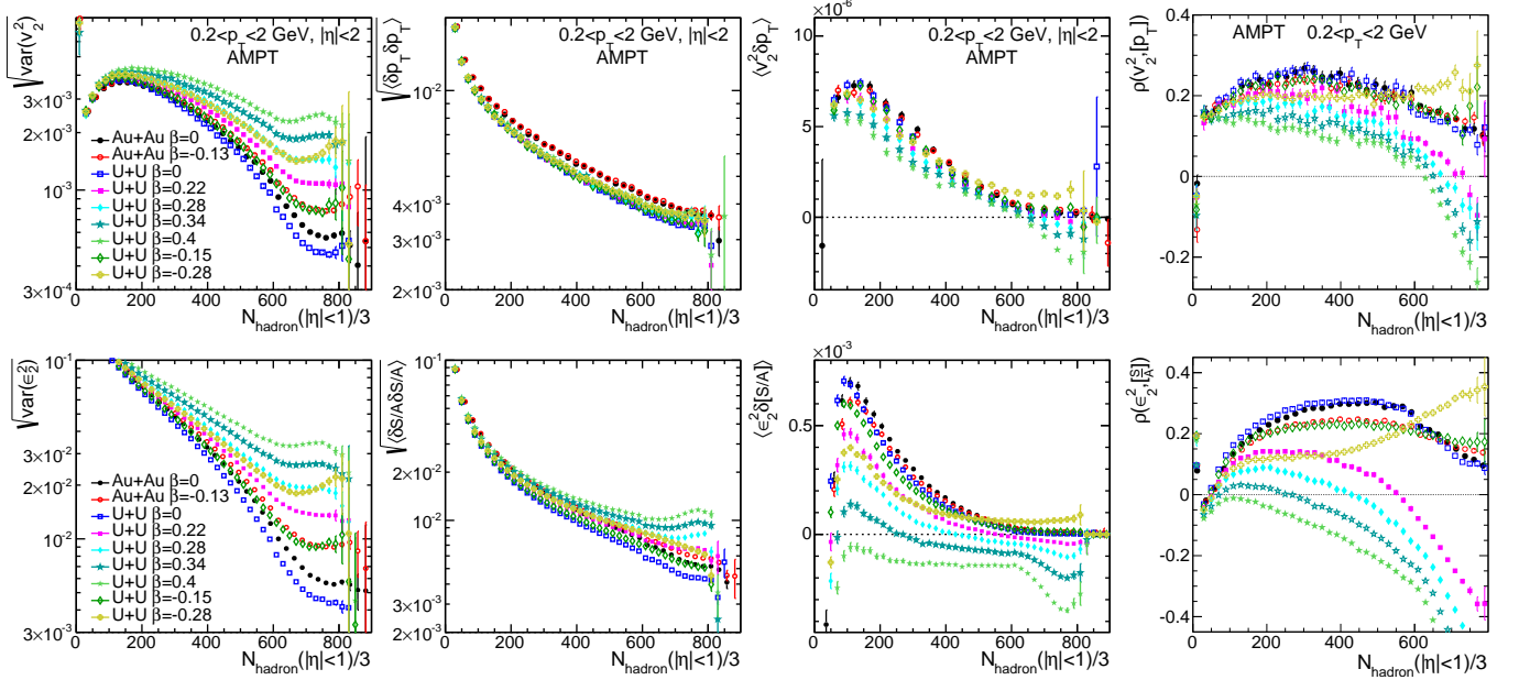
FIG. 7: The N_{\text{hadron}}(|\eta| < 1) dependence of v_2^2 variance (top-left), [p_T] variance (2nd from top-left), flow- [p_T] covariance ( v_2^2 \delta p_T ) (3rd from top-left) and Pearson coefficients \rho(v_2^2, [p_T]) (top-right) in Au+Au and U+U collisions with different deformation parameter \beta . The bottom panels show the corresponding initial-state estimators in the Glauber model. The event class used for averaging is based on N_{\text{hadron}}(|\eta| < 1) .
