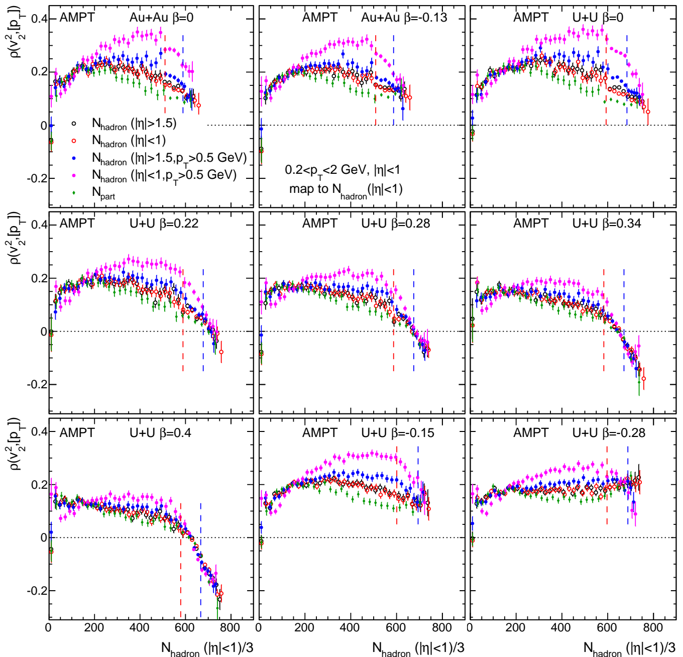
FIG. 8: The centrality dependence of \rho(v_2^2, [p_T]) calculated for hadrons in 0.2 < p_T < 2 \text{ GeV} and |\eta| < 1 and compared between give different event class definitions after mapping to the common x -axis defined by N_{\text{hadron}}(|\eta| < 1)/3 . They are shown separately for Au+Au or U+U collisions with various \beta values as indicated in each panel. The vertical dashed lines indicate the locations for the top 1% and 5% highest N_{\text{hadron}} values.
