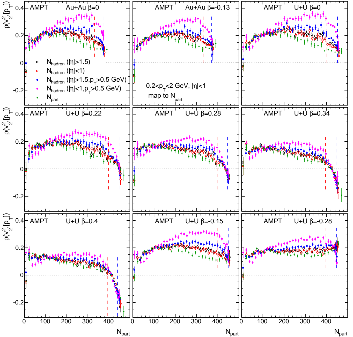
FIG. 6: The N_{\text{part}} dependence of \rho(v_2^2, [p_T]) calculated for hadrons in 0.2 < p_T < 2 GeV and |\eta| < 1 but compared between five different event class definitions after mapping to the common N_{\text{part}} x -axis. They are shown separately for Au+Au or U+U collisions with various \beta values as indicated in each panel. The vertical dashed lines indicate the locations for the 1% and 5% highest N_{\text{part}} values.
