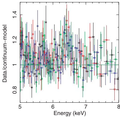
Figure 2. XIS residues from the best-fitting continuum model showing the presence of a 6.4 keV fluorescent line of cold iron. Data from all XIS are shown (XIS0 = black, XIS1 = red, XIS2 = green, XIS3 = blue).
