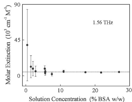
Figure 2. The extracted molar absorption of solvated BSA at 1.56 THz does not vary significantly with concentration. This allows us to focus on more concentrated, more readily measured solutions (~27% BSA [w/w]) in this study.
