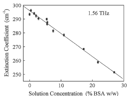
Figure 1. The terahertz absorption of BSA solutions at 1.56 THz varies linearly with solute concentration, consistent with Beer's Law. Of note, the observed extinction decreases with increasing solution concentration, indicating that the terahertz absorption of BSA is not as great as that of the water it displaces.
