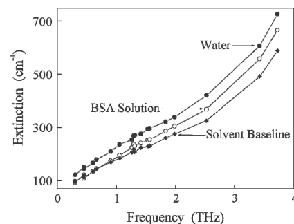
Figure 3. We measure the absorptions of both buffer blanks (●) and BSA solutions (○), and estimate the solvent baseline arising from the bulk water remaining in solution (◆). This baseline is consistently lower than the measured solution extinction, indicating that the BSA solute does not simply displace water but also contributes to the absorption of terahertz radiation. Correction to account for hydration would further reduce the solvent baseline (data not shown).
