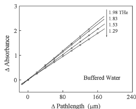
Figure 8. Change in absorbance of liquid sample varies linearly with changing path length. The terahertz absorption of water (shown here) and BSA solutions can be precisely determined from linear fits of the absorbance vs. path length data without precise (and difficult to obtain) absolute path length or absorbance information.
