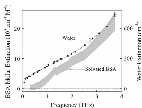
Figure 5. The terahertz absorption spectrum of the solvated protein (shaded area) is very distinct from that of water (▼ [Kindt and Schmuttenmaer 1996] and ● [Xu et al. 2006]). Taken together with the demonstrated Beer's law behavior (Figs. 1,2) and the quantitative agreement between the extinction coefficients of solvated (this study) and dry (Markelz et al. 2000) BSA, this supports the validity of the spectroscopic measurement protocol that we developed and used in this work to extract low-frequency dynamics of a protein against the significantly larger background absorption by liquid water.
