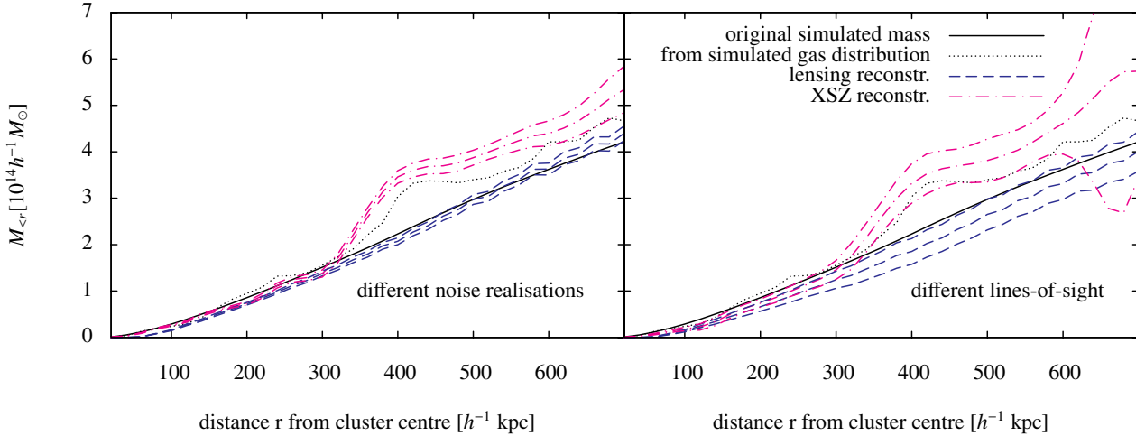
Fig. 6. Mean XSZ and lensing reconstructed cumulative mass profiles M_{<r}(r) and their 1-\sigma errors of merging simulated cluster g51 obtained for different noise realisations ( left panel ) and different lines-of-sight ( right panel ). Profiles of the original simulated mass distribution and the profiles obtained directly from the simulated gas distribution by assuming hydrostatic equilibrium are shown for reference. X-ray, SZ and lensing observations along one line-of-sight but with 50 different noise realisations were used for the reconstructions whose mean and 1-\sigma errors are shown in the left panel. For the right panel we started with a sample of noisy synthetic observations along 50 different randomly oriented lines-of-sight. However we rejected projections for which the merging subhalo is almost directly behind or in front of the main halo (projected distance <200 h^{-1} kpc) as well as one line-of-sight with an inclination of only 2^\circ with respect to the clusters symmetry axis which is too small for a faithful reconstruction. The mean and the 1-\sigma errors of the profiles reconstructed from the observations along the remaining 33 lines-of-sight are shown. For both the different noise realisations and the different lines-of-sight deviations from hydrostatic equilibrium can be reliably detected.
