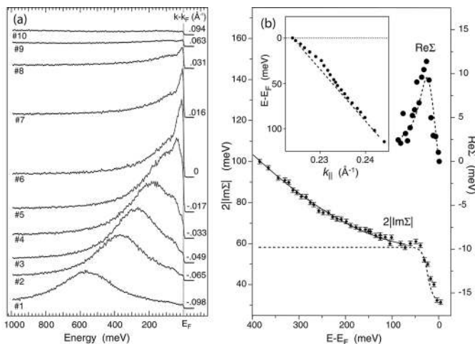
Fig. 15. (a) ARPES spectra for the Be(0001) surface state (from Ref. [107]). (b) Self energy estimated from the Mo(110) surface state ARPES spectra, and corresponding quasiparticle dispersion (inset). Calculated electron-phonon contributions to the real and imaginary part of \Sigma(\mathbf{k}, \omega) are indicated by dotted and dashed lines, respectively (the latter was offset by 26 meV to account for impurity scattering). From Ref. [113].
