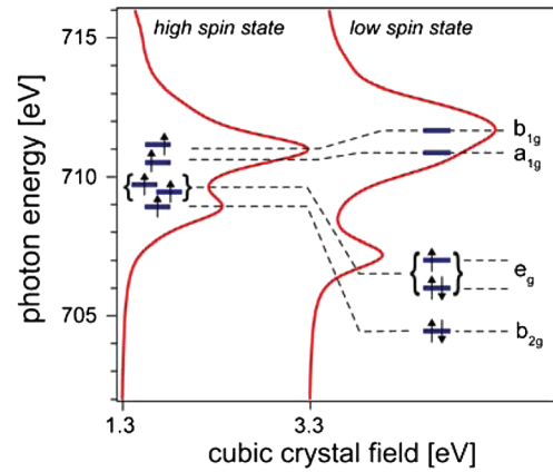
FIG. 2 (color). Calculated Fe L_3 -edge spectra in the HS (left side, hemoglobin case) and the LS case [right side, compare with Fig. 1(b) of Ref. [20]], as a function of the cubic crystal field strength. The Fe d orbital energy levels are also shown for both cases. In the LS state, the b_{2g} and the e_g orbital of lower energy are completely filled and the hole is localized in the other e_g orbital due to a symmetry lowering induced by the \pi -donor ligands [20]. The transition from the 2p_{3/2} core level to the half-filled e_g orbital leads to the peak at about 707 eV. The empty a_{1g} and b_{1g} orbitals yield the main peak and its doublet structure at about 711 and 712 eV. In the HS state, all the orbitals are filled by one electron and can thus contribute to the XA spectrum. The b_{2g} and e_g orbitals lead to the peak at about 709 eV and the a_{1g} and b_{1g} orbitals to the main peak at 711 eV.
