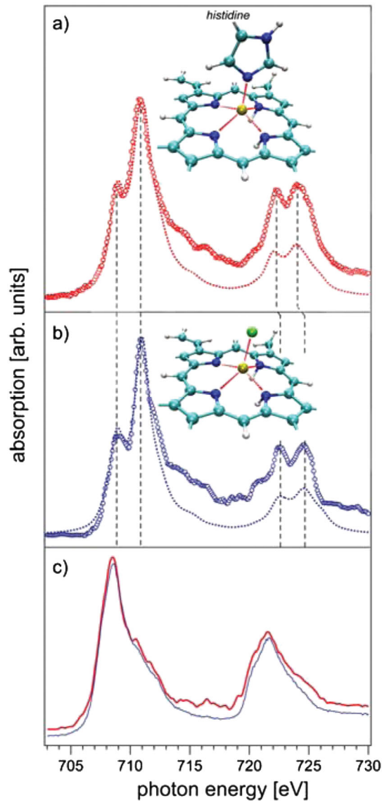
FIG. 1 (color). Experimental Fe L_{2,3} edge XA spectra of hemoglobin (a), and hemin (b) in solution (3 mM), recorded with 200 meV resolution, along with the molecular structure of the metalloporphyrin. The L_3 edge lies in the \sim 708 – 716 eV region, while the L_2 -edge lies in the \sim 720 – 726 eV region. Panel (c) presents the experimental spectra for hemoglobin (red thick line) and hemin (blue line) in powder form. The dotted lines in (a) and (b) represent the simulated Fe L_{2,3} edge spectra calculated using the ligand field multiplet (LMF) theory (see text and supplementary material [19] for details).
