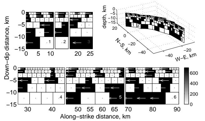
Figure B1. Synthetic slip model used in the resolution test.
