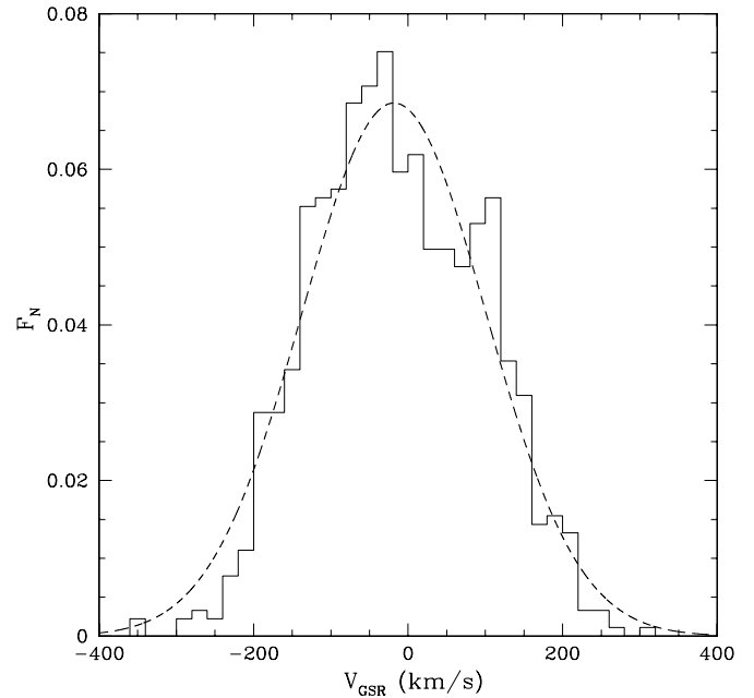
Figure 23. Distribution of RRab radial velocities relative to the Galactic standard of rest ( V_{\text{GSR}} ). This histogram contains values for the 905 CSS RRab's with SDSS DR8 radial velocity measurements. The Gaussian fit to the distribution is also plotted. The plot presents the fractional number of objects, F_N .
