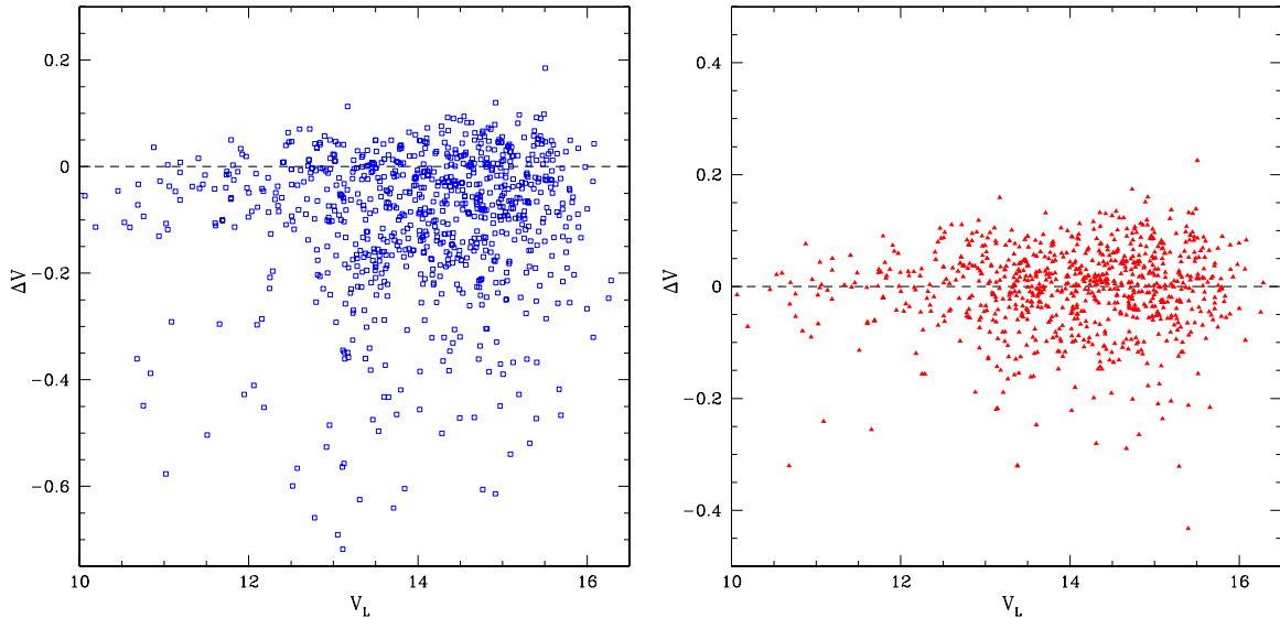
Figure 2. Comparison of CSS V magnitudes with Landolt magnitudes for standard stars. The left plot shows the difference in magnitudes before color corrections and the right plot shows the difference after color corrections have been applied.
