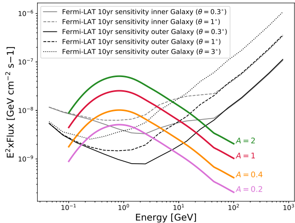
FIG. 1. Gamma-ray fluxes calculated for different values of the A parameter, For comparison, the Fermi -LAT flux sensitivities for different regions of the sky and for different angular extensions of sources are shown.
