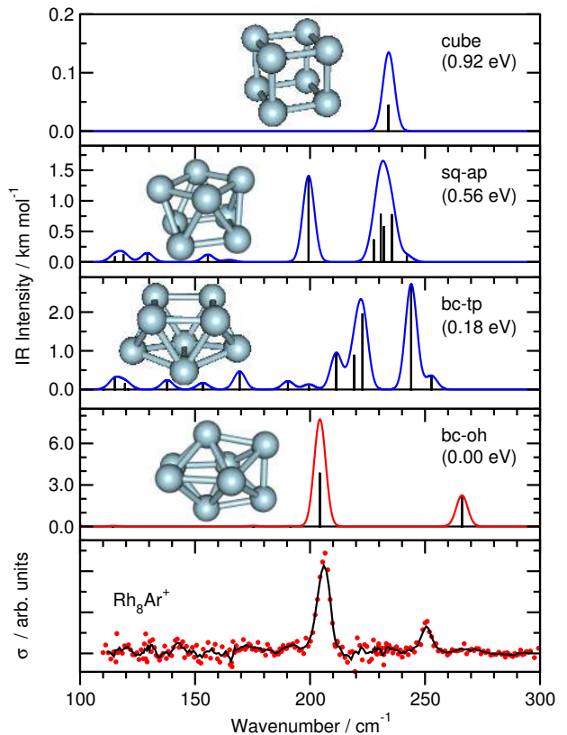
FIG. 3: FIR-MPD spectrum of \text{Rh}_8\text{Ar}^+ and calculated spectra of \text{Rh}_8^+ at the PBE1/LANL2DZ level.
