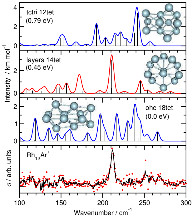
FIG. 9: Experimental spectrum of \text{Rh}_{12}\text{Ar}^+ and calculated spectra of low-energy \text{Rh}_{12}^+ isomers.
