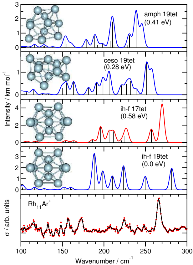
FIG. 8: Experimental spectrum of \text{Rh}_{11}\text{Ar}^+ and calculated spectra of \text{Rh}_{11}^+ .
