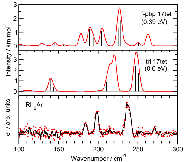
FIG. 5: The spectra of the tri and f-pbp isomers calculated at the TPSSh/def2-TZVP level.
