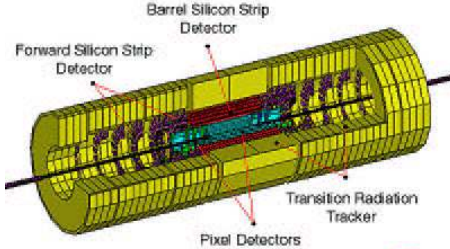
Figure 1.8: A cut-away view of the ATLAS inner detector is shown [Atl97a]. The outer radius of the inner detector is 1.15 m.
