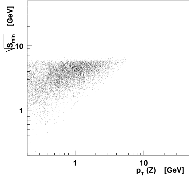
Figure 2.9: The kinematics of \Phi -space Veto method event candidates which have been vetoed because they lie below the s_{\text{zero}} boundary are plotted in the P_Z^T vs. \sqrt{s_{\text{min}}} plane. The largest P_Z^T of a vetoed candidate event is 5.5 GeV. The process is p\bar{p} \rightarrow Z^0 + X \rightarrow l^+l^- + X at 2 TeV with the lepton-pair mass restricted to 66-116 GeV.
