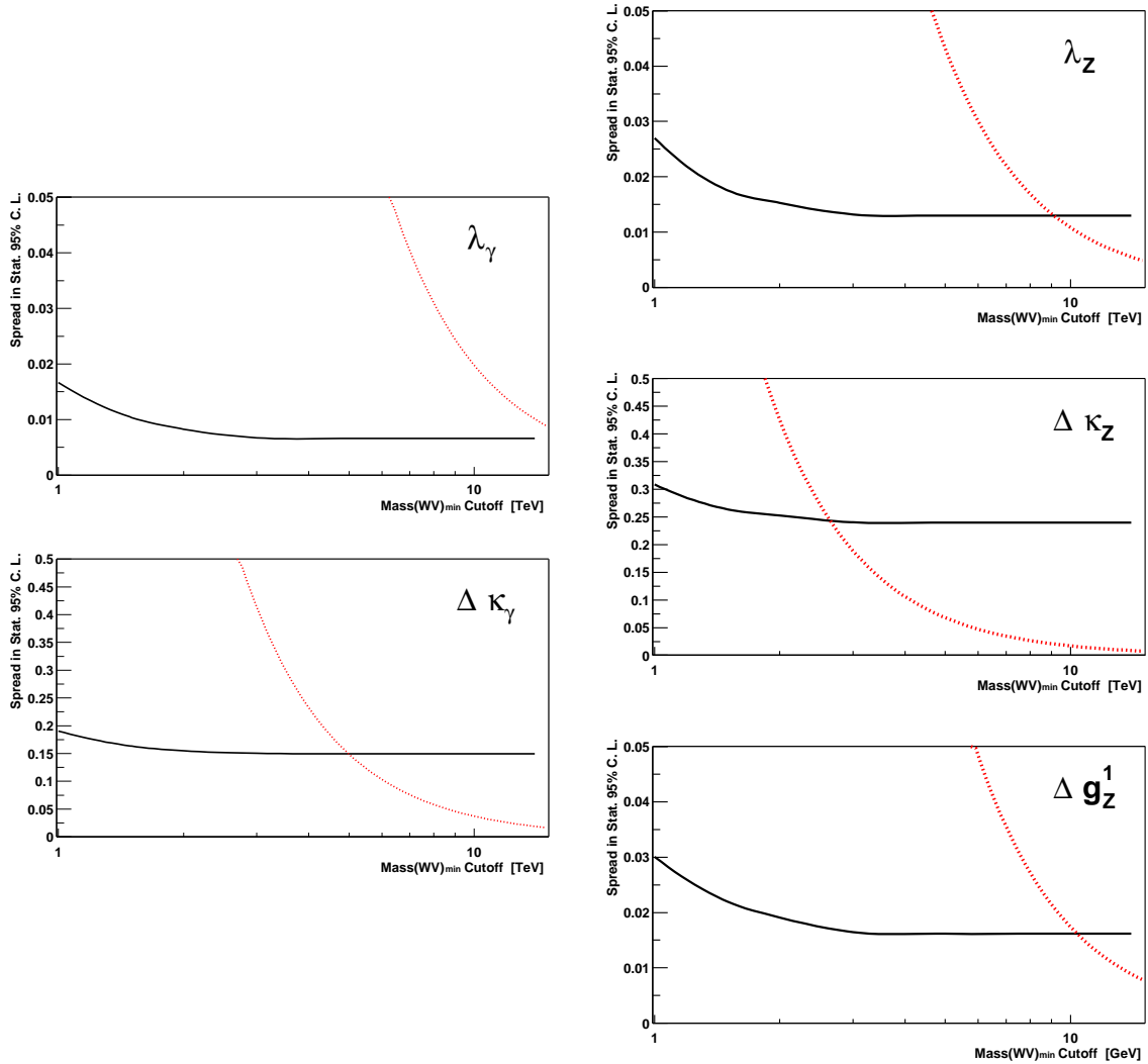
Figure 5.15: The spread in statistical 95% confidence intervals (solid lines) are shown as a function the diboson mass cutoff, which is used as a selection criteria for events included in the analysis. Limits for the W\gamma production parameters are shown at left and the WZ production parameters at right, assuming an integrated luminosity of 30 \text{ fb}^{-1} at the LHC. The dotted lines indicate the approximate Born level unitarity limits from Eq. 3.14. The region above the solid line is excluded by the experiment, while the region to the right of the dotted line is excluded by unitarity.
