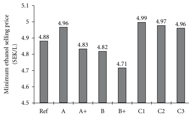
FIGURE 4: Minimum ethanol selling price. Carbon source A: pretreated liquid fraction, B: pretreated liquid fraction and molasses and C: pretreated liquid fraction and pressed pretreated slurry with a total WIS content of 1%, 2% and 3%; +: 1.5-fold specific activity; Ref: reference case with purchased enzyme preparation.
