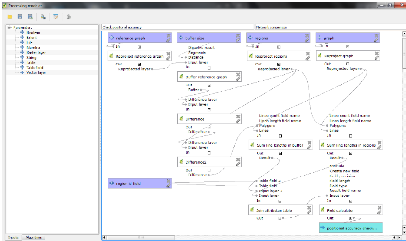
Figure 8. Positional accuracy comparison model; updated version of the model published in [17].
