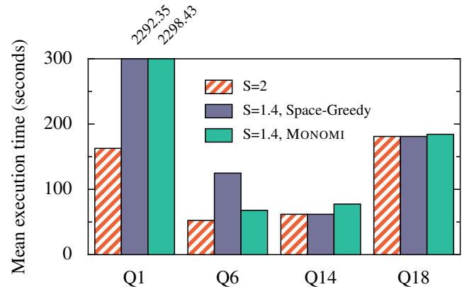
Figure 9: Execution times of queries that were affected by reducing the space budget from S = 2 to S = 1.4 .
