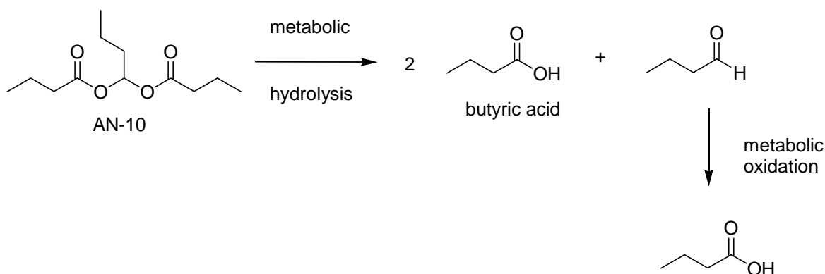
Figure 45. Metabolic hydrolysis of AN-10.
