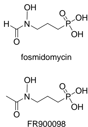
Figure 15. Chemical structures of fosmidomycin and FR900098.
