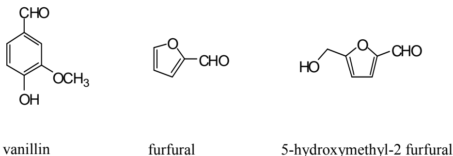
Figure 47. Some aldehyde derivatives with potent antisickling effect.
