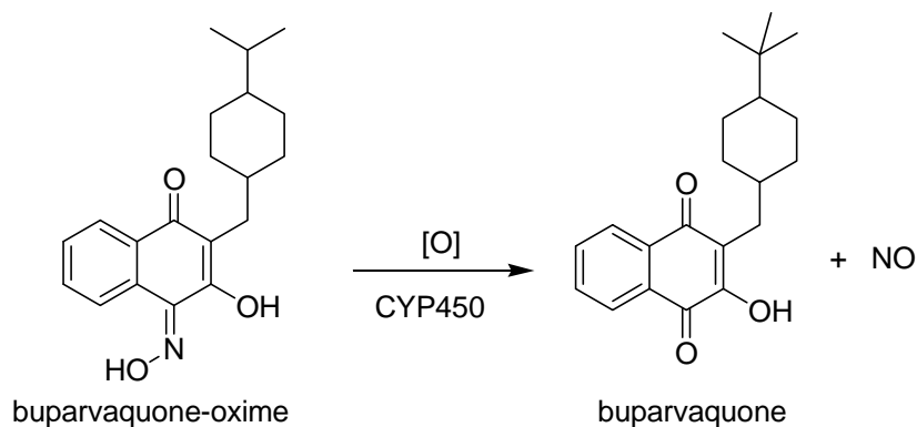
Figure 12. The conversion of buparvaquone-oxime into buparvaquone by enzymatic oxidation and release of NO.
