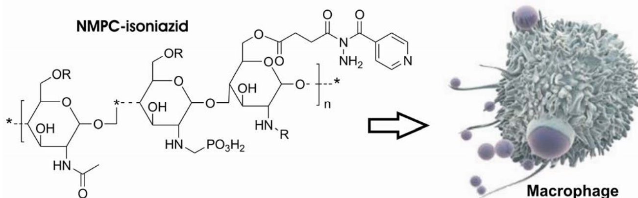
Figure 42. Chitosan-Isoniazid hemisuccinate.
