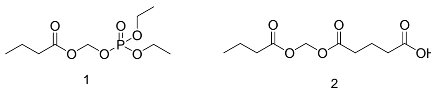
Figure 46: Neutral (1) and acid (2) derivatives of butyric acid.
