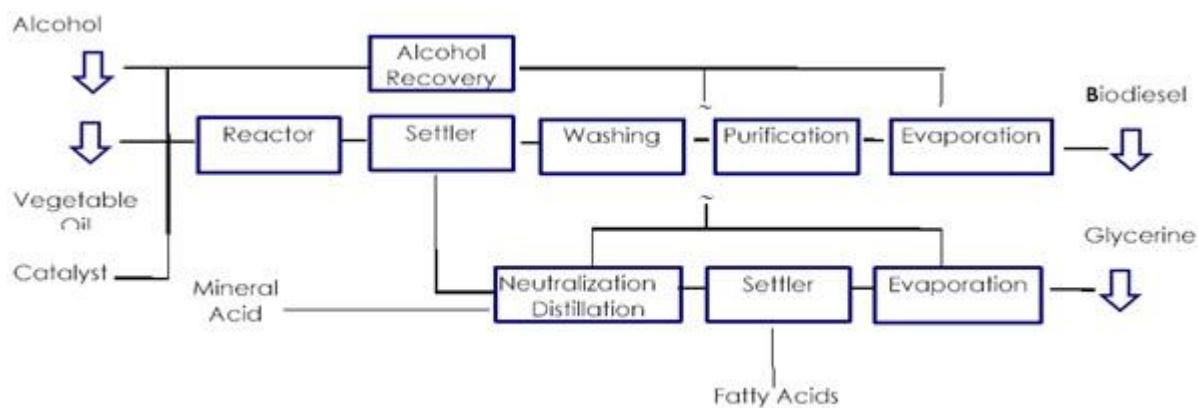
Figure 3. Flow sheet of biodiesel production [41].
