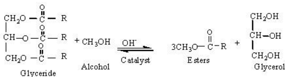
Figure 2. Transesterification reactions.
