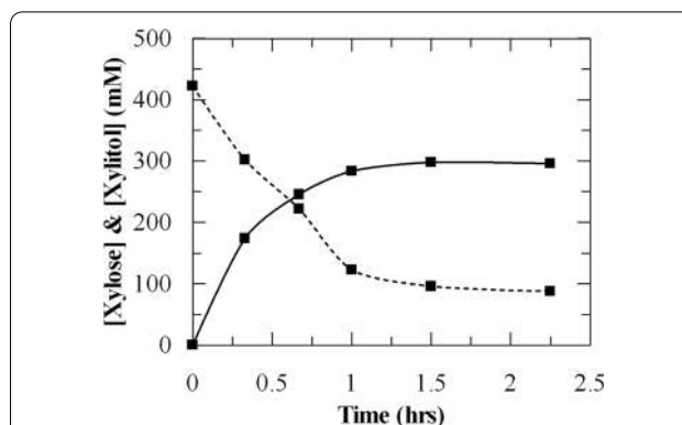
Fig. 5 Xylitol production by PsXYL1 + GDH 4000–4 from a hemicelluloses hydrolysate. The PsXYL1 + GDH 4000–4 cells used in this experiment was originated from a 10-L fed-batch fermentation. One L of hemicelluloses hydrolysate (pH 7.0) was incubated with 100 mg/mL PsXYL1 + GDH 4000–4 cells at 30 °C. Solid lines represent xylitol production; dashed lines represent D-xylose consumption. The data shown in the figure is the average of 3 values. All the values are within the 5% SD
