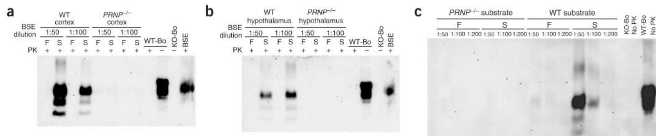
Figure 4. In vitro propagation of PrP BSE and PrP TME in PRNP -/- and PRNP +/+ wild-type (WT) cattle brain homogenates. (a,b) In vitro propagation of PrP BSE in 10% homogenates from cortex (a) or hypothalamus (b) . (c) In vitro propagation of PrP TME in 10% homogenates from cortex (c) . The pathological form of the prion protein, PrP BSE or PrP TME , in the inoculum, was derived from BSE- or TME-affected cattle, respectively. We used 1:50, 1:100 and 1:200 dilutions of the infectious material. Samples were either frozen immediately after mixture (F) or subjected to 48 PMCA amplification cycles (S). The appearance of PrP BSE or PrP TME was assessed by western blot analysis after proteinase K (PK) digestion. Samples from PRNP +/+ wild-type (WT-Bo), PRNP -/- (KO-Bo) cattle (substrates) and the BSE-positive control brain homogenate (inoculum) are shown for comparison with and without PK treatment.
