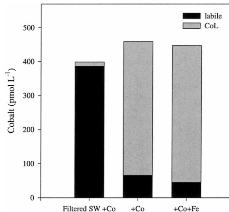
Fig. 6. Cobalt speciation on bottle incubation samples after 5 d. The control treatment represents a filtered seawater control amended with Co and allowed to incubate under the same conditions as the enrichment experiment.
