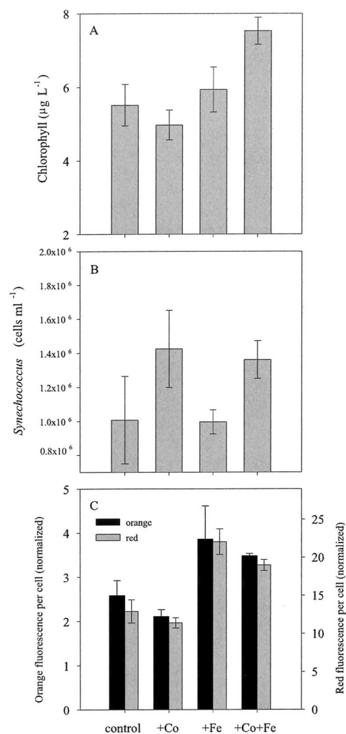
Fig. 5. (A) Bottle incubation chlorophyll results under cobalt, (+Co), iron (+Fe), and combined Co and Fe additions (+Co +Fe), relative to an unamended control. \text{CoCl}_2 and \text{FeSO}_4 additions were 420 \text{ pmol L}^{-1} and 0.83 \text{ nmol L}^{-1} , respectively. Error bars represent standard deviation of triplicate bottles. (B) Synechococcus cell numbers, and (C) Synechococcus red and orange fluorescence per cell, normalized to added fluorescent beads. Results reflect 2 d of incubation.
