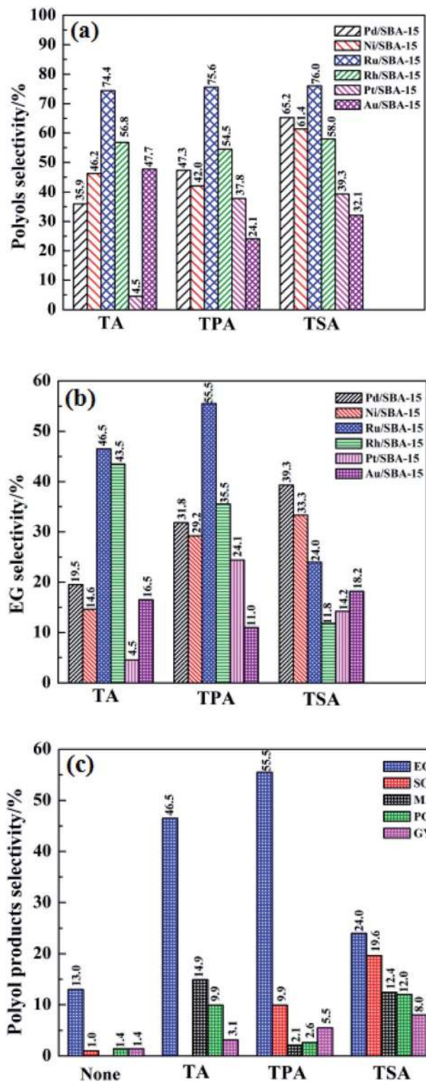
Fig. 5 The selectivity of the polyols and EG as well as the main products for the catalytic conversion cellulose (a): polyols selectivity; (b): EG selectivity; (c): product selectivity). Reaction conditions: 0.5 g of cellulose; 0.1 g of M/SBA-15; 0.02 g of W compound; 25 mL H 2 O; reaction temperature, 245 °C; reaction time, 4 h; H 2 pressure, 5 MPa.
