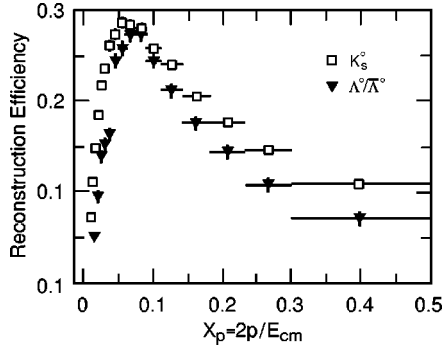
FIG. 7. The simulated reconstruction efficiencies as a function of x_p for K_s^0 (squares) and \Lambda^0/\bar{\Lambda}^0 (triangles). The charged decay branching ratios are included in the efficiency. The discontinuity in the \Lambda^0/\bar{\Lambda}^0 reconstruction efficiency at x_p=0.04 is due to the invariant-mass cut to remove the low-momentum K_s^0 background.
