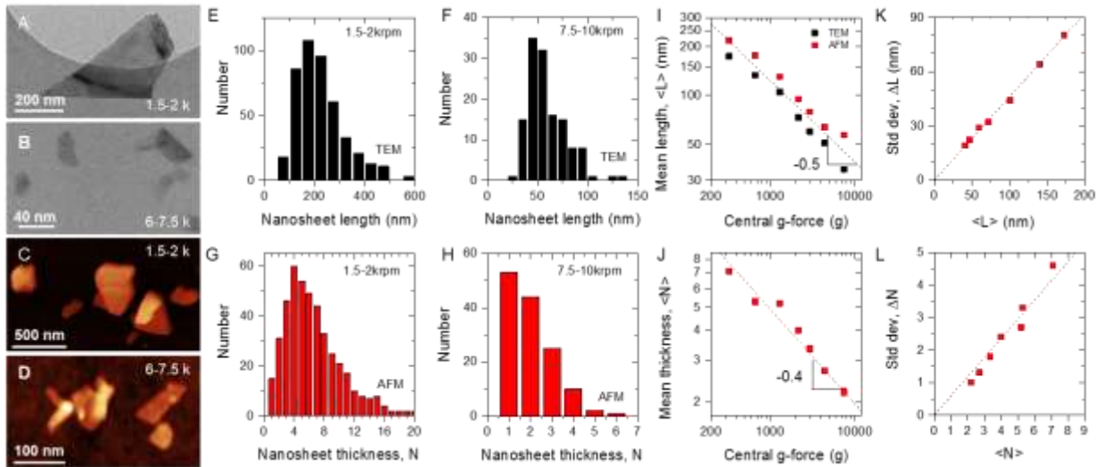
Figure 2: Microscopic characterization of size-selected \text{WS}_2 nanosheets. A-D) TEM (A-B) and AFM (C-D) images of nanosheets, size-selected with upper and lower centrifugation speeds of (A&C) 1.5 krpm and 2 krpm and (B&D) 6 krpm and 7.5 krpm respectively. E-J) Statistical analysis of dimensions of nanosheets extracted from images such as those in A-D. This is presented as histograms representing data for lateral nanosheet size measured by TEM (E-F) and nanosheet thickness (number of monolayers per nanosheet, N ) determined by AFM (G-H). Data is shown for two combinations of centrifugation speed, 1.5-2 krpm and 6-7.5 krpm. I, J) Data extracted from histograms for a range of centrifugation conditions. Mean values of I) nanosheet length, \langle L \rangle , and J) nanosheet thickness, \langle N \rangle , as a function of the central centrifugation acceleration, presented as central g -force. K-L) Standard deviation of nanosheet length (K) and thickness (L) plotted versus mean length and thickness respectively. The dashed lines in K and L represent \Delta L / \langle L \rangle = 0.46 and \Delta N / \langle N \rangle = 0.59 respectively.
