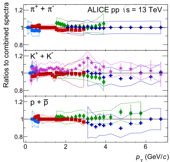
bined spectra as a function of p_T for \pi^\pm (top), K^\pm (middle), and p(\bar{p}) (bottom). Only the p_T -range where the analyses overlap is shown. The vertical bars indicate statistical uncertainties while the bands show the uncorrelated systematic uncertainties
