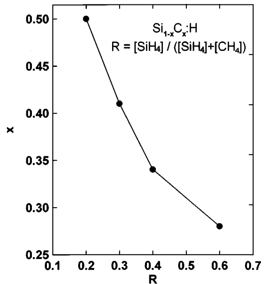
FIG. 1. Dependence of the carbon concentration x on the precursor gas mixture R . R = [\text{SiH}_4] / ([\text{SiH}_4] + [\text{CH}_4]) for the second series of powders.
