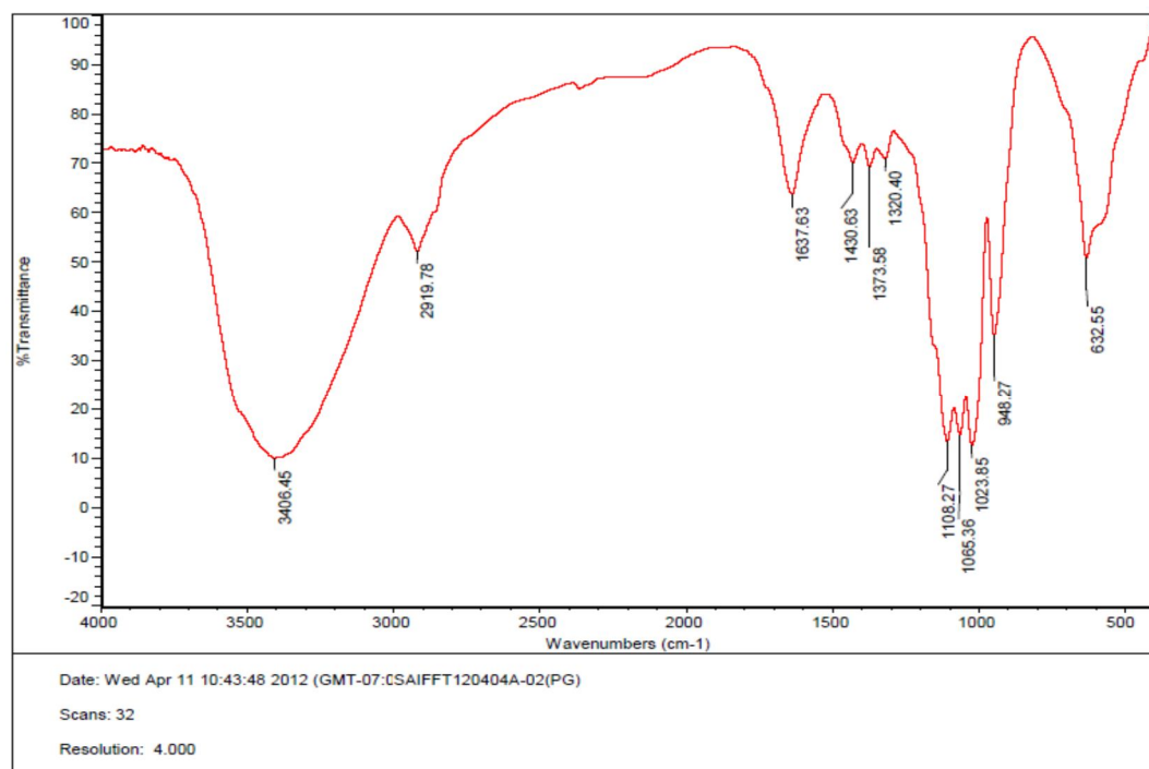
Figure 3 FTIR analysis of extracted PHA from SPY-1
