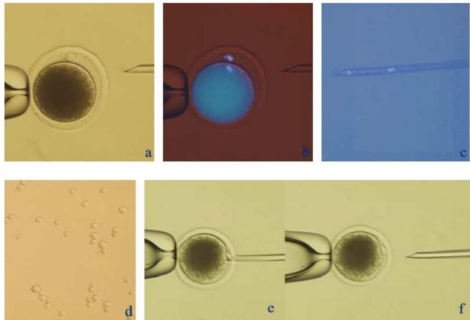
FIG. 1. Steps in the SCNT of dromedary camel. a ) A mature oocyte with a visible polar body held with a pipette. b ) Determining the location of metaphase chromosomes by a very short (1–2 sec) exposure to UV light. c ) Exposing the pipette to UV light to confirm the presence of both metaphase and polar body chromatin. d ) Donor cells after trypsinization and washing. e, f ) Injection of the donor cell into the perivitelline space of the enucleated oocyte. Original magnification \times 200 .
