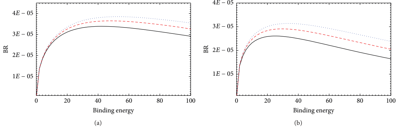
FIGURE 2: (a) The dependence of the branching ratios of Y(5S) \rightarrow \gamma X_b on \epsilon_{X_b} using monopole form factors with \alpha = 2.0 (solid lines), \alpha = 2.5 (dashed lines), and \alpha = 3.0 (dotted lines), respectively. (b) The dependence of the branching ratios of Y(5S) \rightarrow \gamma X_b on \epsilon_{X_b} using dipole form factors with \alpha = 2.0 (solid lines), \alpha = 2.5 (dashed lines), and \alpha = 3.0 (dotted lines), respectively. The results with binding energy up to 100 MeV might make the molecular state assumption inaccurate.
