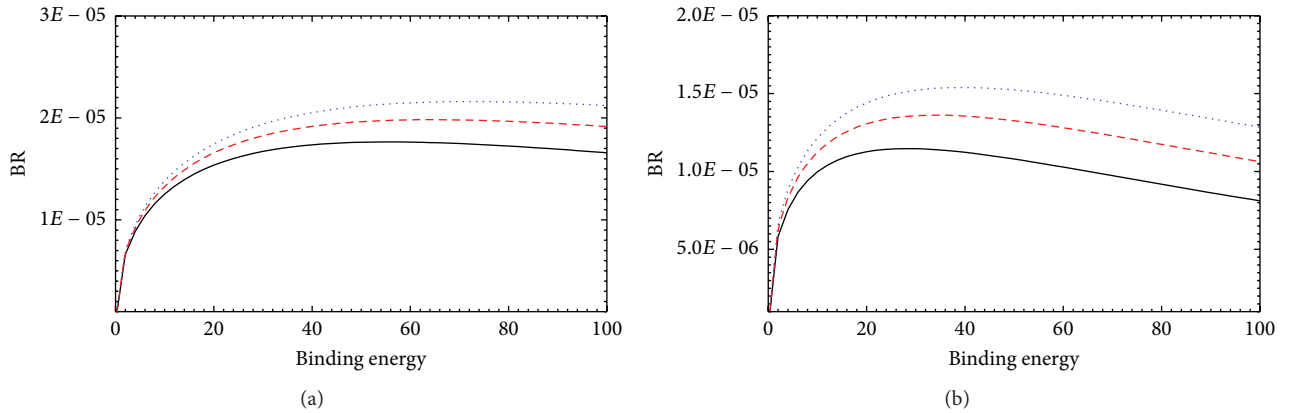
FIGURE 3: (a) The dependence of the branching ratios of Y(6S) \rightarrow \gamma X_b on \epsilon_{X_b} using monopole form factors with \alpha = 2.0 (solid lines), \alpha = 2.5 (dashed lines), and \alpha = 3.0 (dotted lines), respectively. (b) The dependence of the branching ratios of Y(6S) \rightarrow \gamma X_b on \epsilon_{X_b} using dipole form factors with \alpha = 2.0 (solid lines), \alpha = 2.5 (dashed lines), and \alpha = 3.0 (dotted lines), respectively. The results with binding energy up to 100 MeV might make the molecular state assumption inaccurate.
