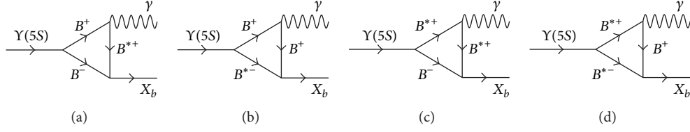
FIGURE 1: Feynman diagrams for X_b production in Y(5S) \rightarrow \gamma X_b under B\bar{B}^* meson loop effects.
