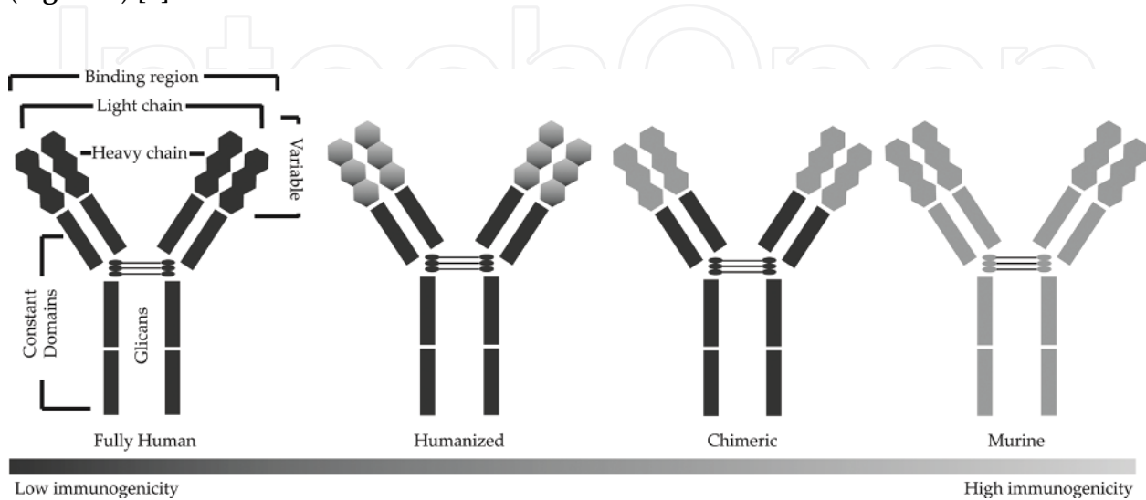
Figure 1. Schematic overview of a monoclonal antibody, showing their heavy and variable chain.
