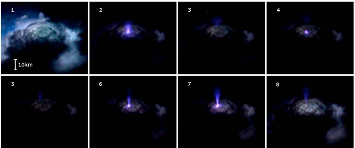
Figure 3. The pulsating blue jet from the top of the Northern cloud. Frame 1 is the first of the time sequence. It serves as a reference frame to illustrate the structure of the cloud. Frames 2–8 show the pulsating blue jet.
