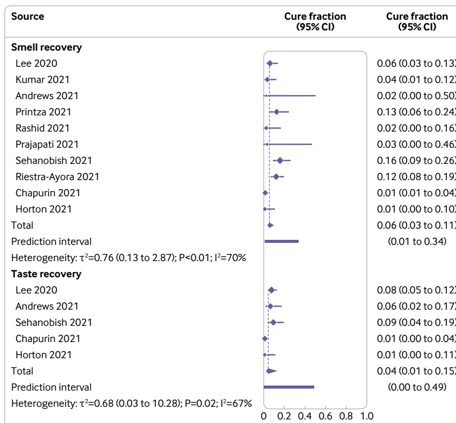
Fig 3 | Random effects meta-analysis of Weibull non-mixture cure fraction for individual studies of persistent smell and persistent taste dysfunction after covid-19. 1 corresponds to 100%. Stretched purple diamonds are the pooled proportion with confidence intervals (CIs) for each random effects meta-analysis; symmetrical purple diamonds with horizontal lines are the study estimate with CIs, where diamond sizes reflect the relative weight apportioned to studies in the meta-analysis. The restricted maximum likelihood estimator was used to estimate \tau^2 , and the Hartung-Knapp adjustment was applied to test statistics and CIs
