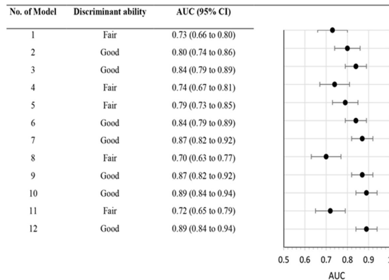
Fig. 3 Discrimination performance in internal validation models
