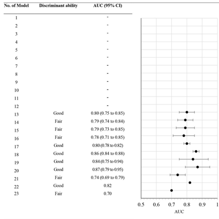
Fig. 2 Discrimination performance in development models
