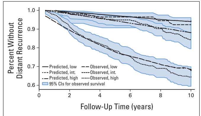
Fig 5. Predicted versus observed time to distant recurrence (Kaplan-Meier curves plus 95% CIs) for the tertiles of the combined score in the Nottingham data. int., intermediate.
