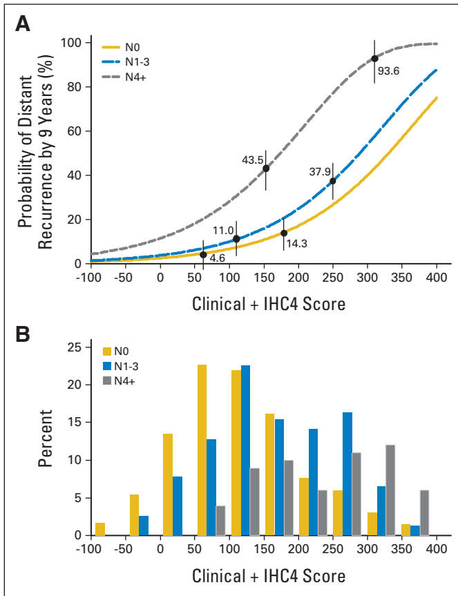
Fig 4. Predicted 9-year distant recurrence probabilities for different nodal status groups according to the sum of the IHC4 score (score for four immunohistochemical markers: estrogen receptor, progesterone receptor, human epidermal growth factor receptor 2, and Ki-67) and clinical score (after removing nodal status term) and histogram for clinical score + IHC4 score for each nodal status. The predicted 9-year distant recurrence rates for a patient at the 25th and 75th percentile of the score for each nodal category are indicated.
