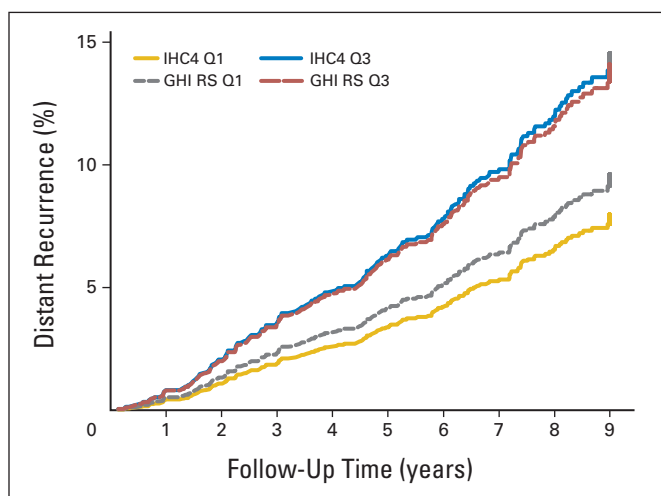
Fig 3. Example of predicted time to distant recurrence for a node-negative patient age \geq 65 years with a poorly differentiated 1- to 2-cm tumor treated with anastrozole who is at either the 25th (quartile 1 [Q1]) or 75th (Q3) percentile of the IHC4 score [score for four immunohistochemical markers: estrogen receptor, progesterone receptor, human epidermal growth factor receptor 2, and Ki-67] or the Genomic Health recurrence score (GHI-RS).
