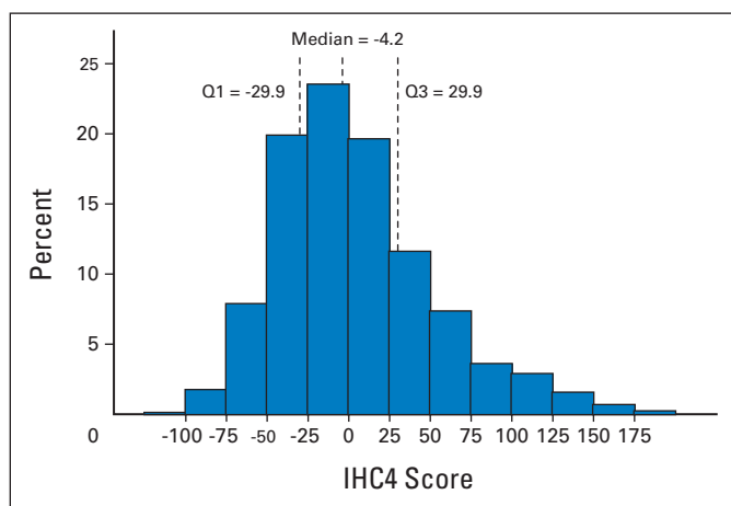
Fig 2. Histogram of IHC4 score (score for four immunohistochemical markers: estrogen receptor, progesterone receptor, human epidermal growth factor receptor 2, and Ki-67) with median and interquartile range for all patients (see Appendices 1 and 2, online only). Q, quartile.
