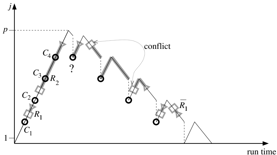
Figure 11. The scope for resource R_1 is benign while the scope for resource R_2 straddles checkpoints and causes problems.
