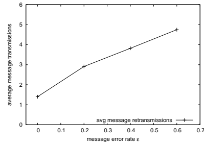
Fig. 16: Performance of TeenyLIME reliable protocol.
