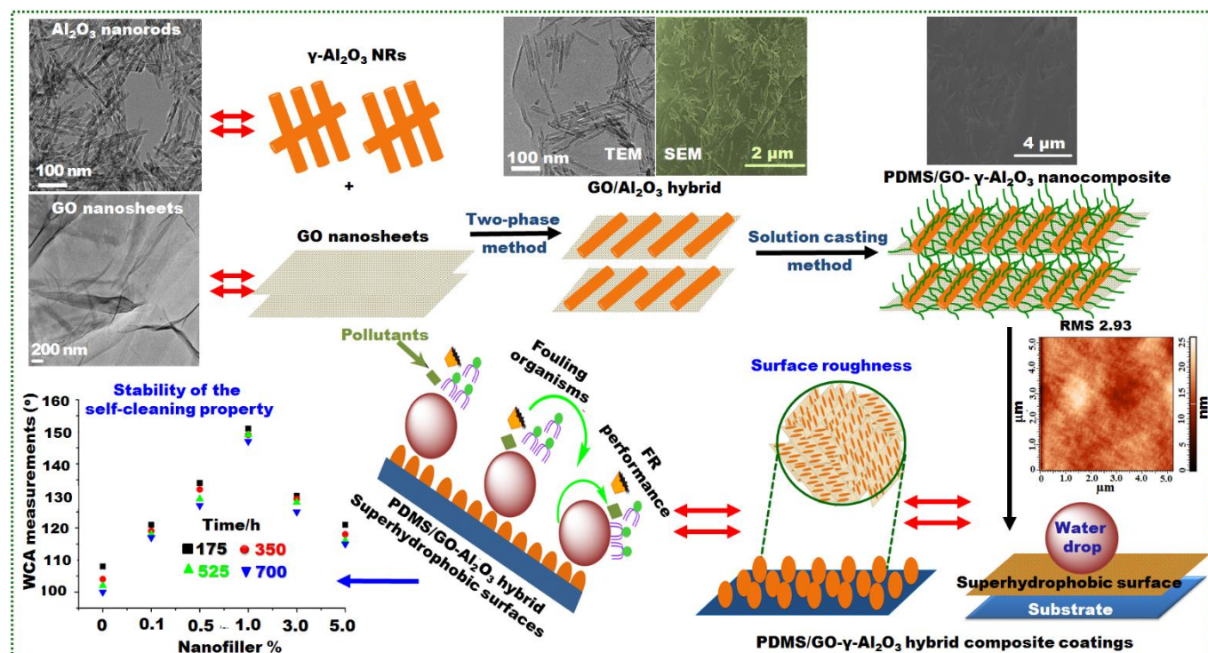
Figure 7. Schematic illustration of the hybridization between GO nanosheets (synthesized through a modified Hummer's method) and \gamma -Al 2 O 3 (prepared and controlled through hydrothermal and calcination methods) to yield GO/ \gamma -Al 2 O 3 hybrid. Inside the TEM images of GO sheets, \gamma -Al 2 O 3 nanorods and GO/ \gamma -Al 2 O 3 hybrid were indicated. Designing superhydrophobic PDMS/GO- \gamma -Al 2 O 3 nanorods hybrid composites was carried out through a solution casting method followed by hydrosilation curing to yield self-cleaning and FR coating surface. AFM and SEM of the nanocomposite surface indicated the surface roughness; which was represented in through discussing the FR mechanism. The FR effectiveness is enhanced by well-dispersion of GO/ \gamma -Al 2 O 3 hybrid nanofillers. Also, thermal stability of the WCAs of the nanocomposites was compared among a series of nanofiller concentrations and showed the highest effectiveness for well-dispersed (1 wt.%) nanofillers. 146 Copyright 2018, reproduced with permission from Elsevier.
